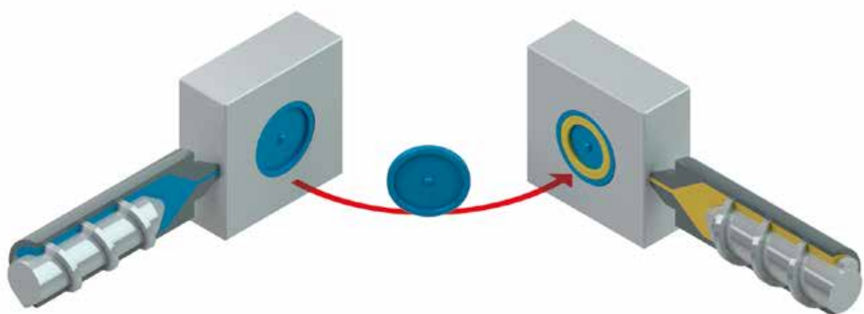
2K injection molding on two injection molding machines
